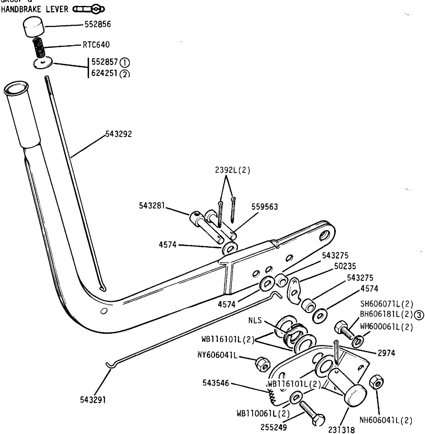
Handbrake lever assembly 624252
